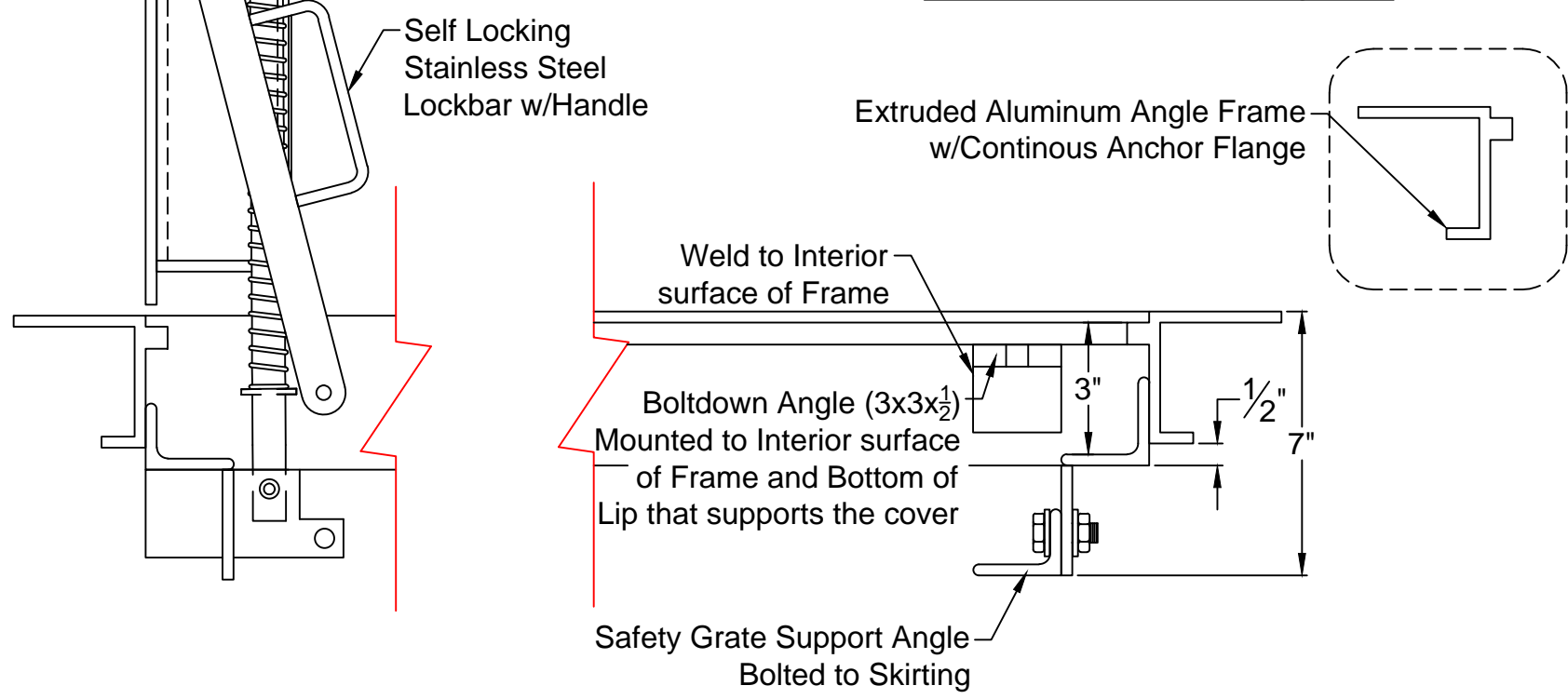
Hatch Side Elevation w/Safety Gate
